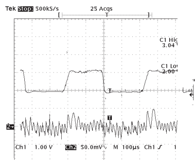
Line Transient Response @100mA Load
