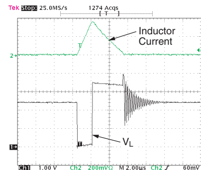
Inductor Current and Switching Node Voltage
