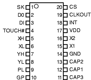
MK715 20 pin SSOP
