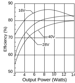
MHF2812S Efficiency FIGURE 3
