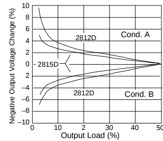
Condition A: 50% Load Pos. Vout, 50% to 20% Neg. Vout Condition B: 50% Load Neg. Vout, 50% to 20% Pos. Vout MHF Negative Output Voltage Cross Regulation
