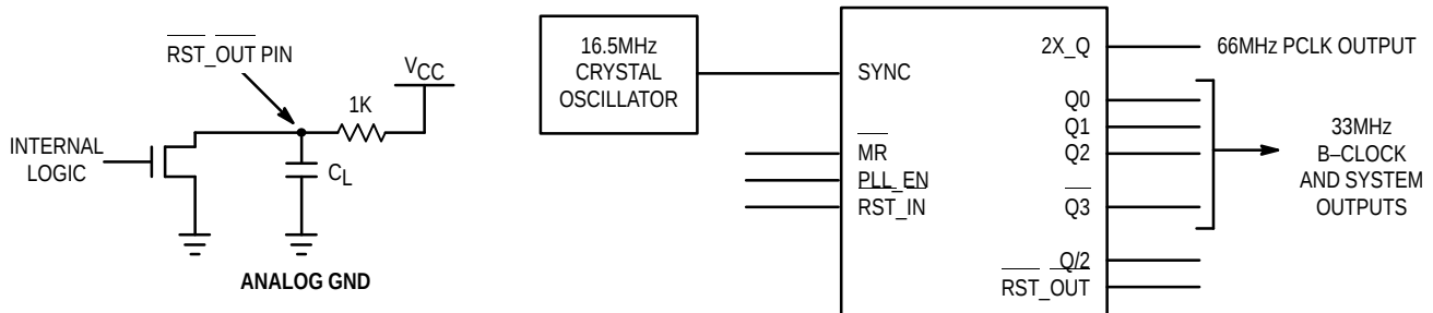
Figure 4. RST_OUT Test Circuit
