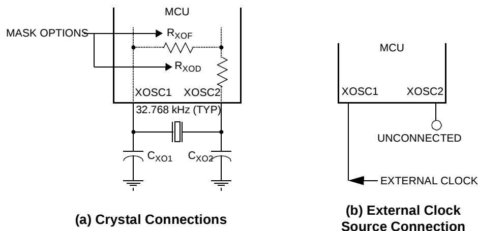
Figure 1-4. Oscillator Connections
