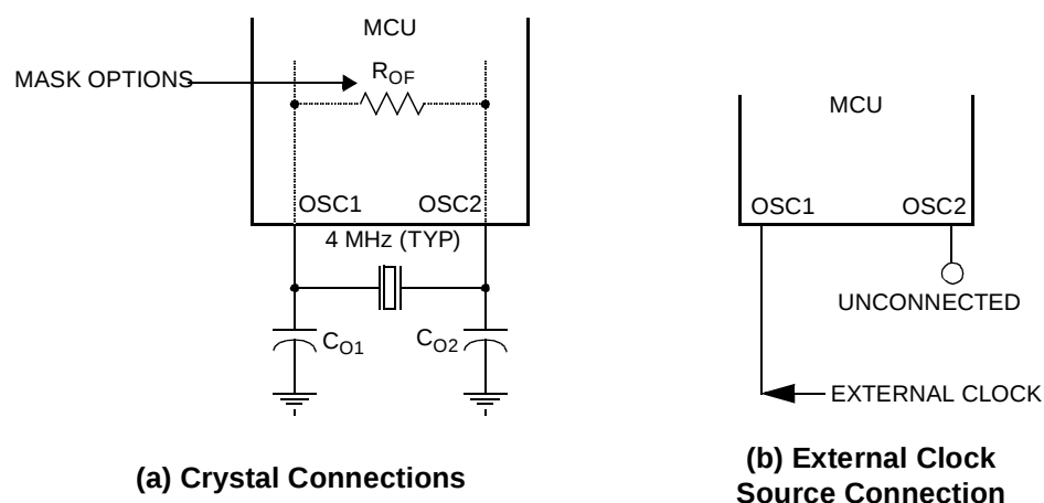
Figure 1-3. Oscillator Connections
