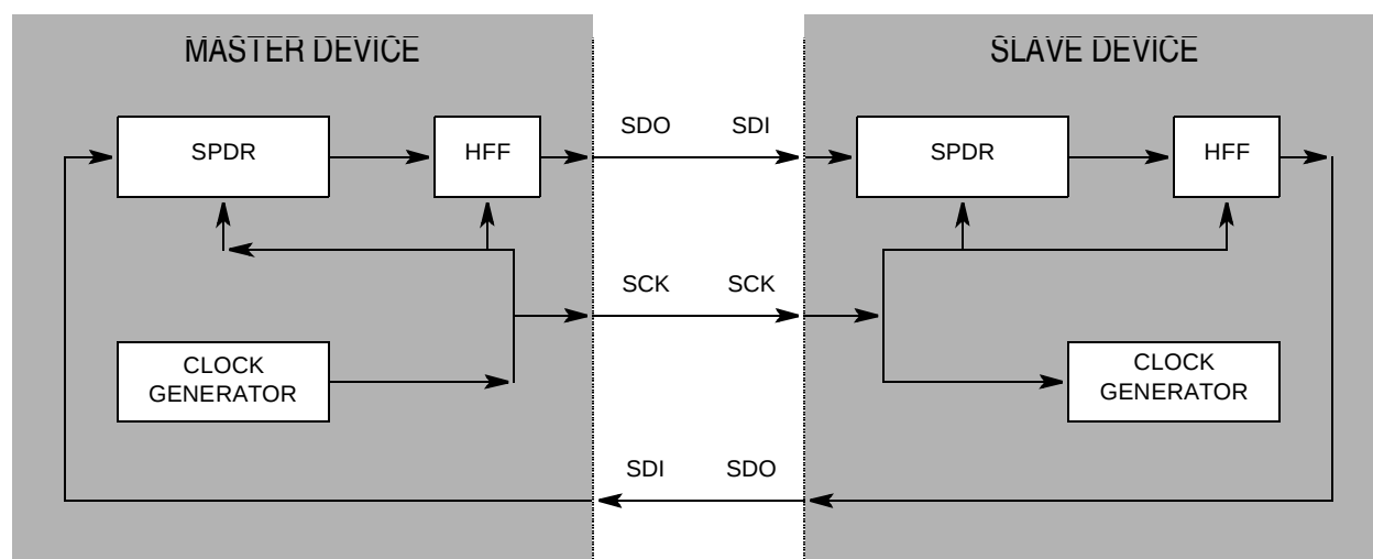
Figure 8-1. SSPI Master-Slave Interconnection
