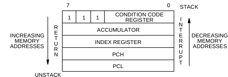
Figure 3-1. Programming Model
