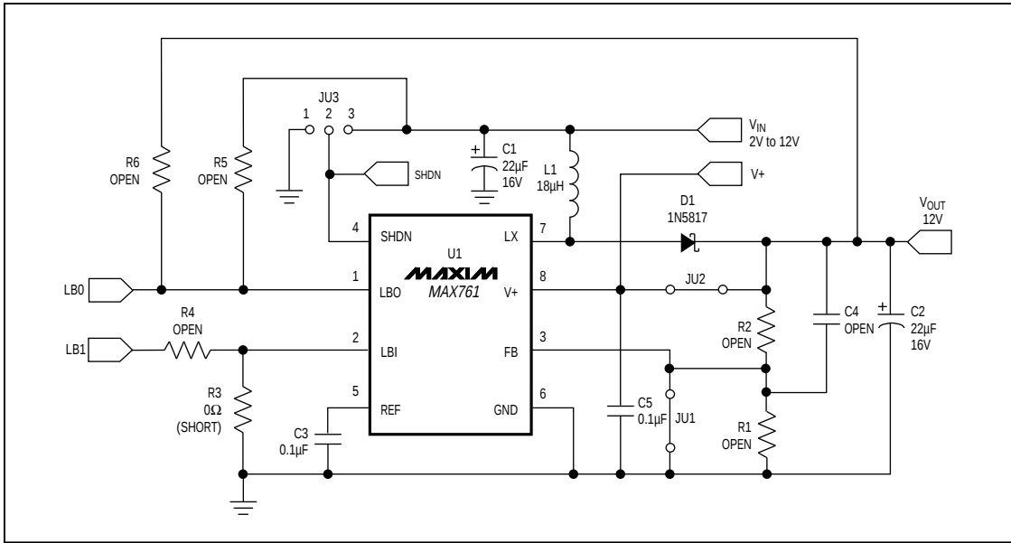
Figure 1. MAX761 EV Kit Schematic Diagram
