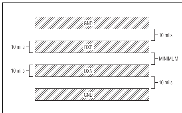
Figure 5. Recommended DXP-DXN PC Board Traces
