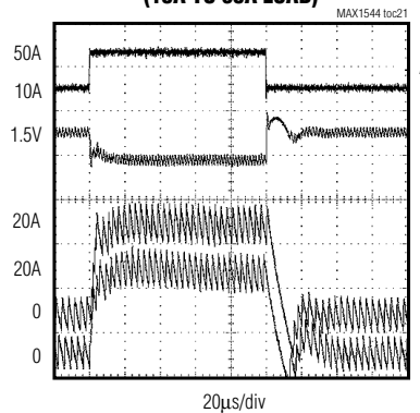
1.50V LOAD TRANSIENT (10A TO 50A LOAD)
