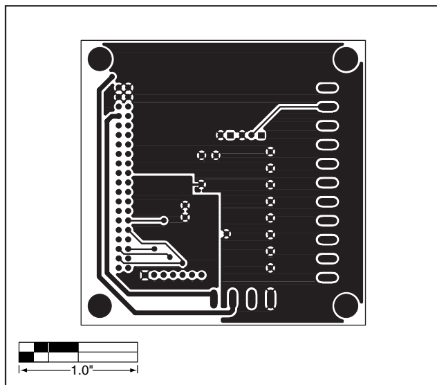
Figure 4. MAX1280 EV Kit PC Board Layout—Solder Side
