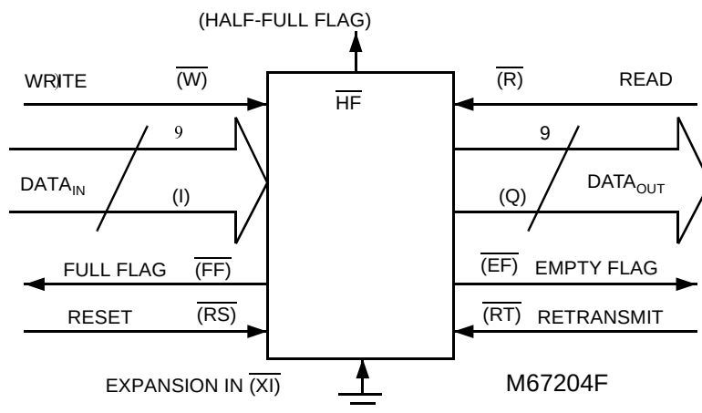
Figure 2. Block Diagram of Single 4096 \times 9.
