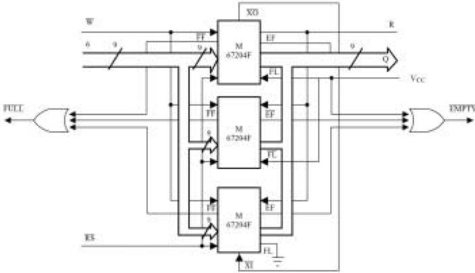
Figure 4. Block Diagram of 12288 × 9 FIFO Memory (Depth expansion).
