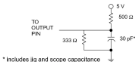
Figure 7. Output Load
