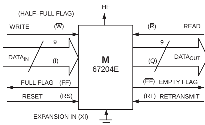
Figure 2. Block Diagram of Single 4K \times 9 FIFO.
