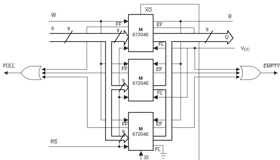
Figure 4. Block Diagram of 12288 \times 9 FIFO Memory (Depth expansion).
