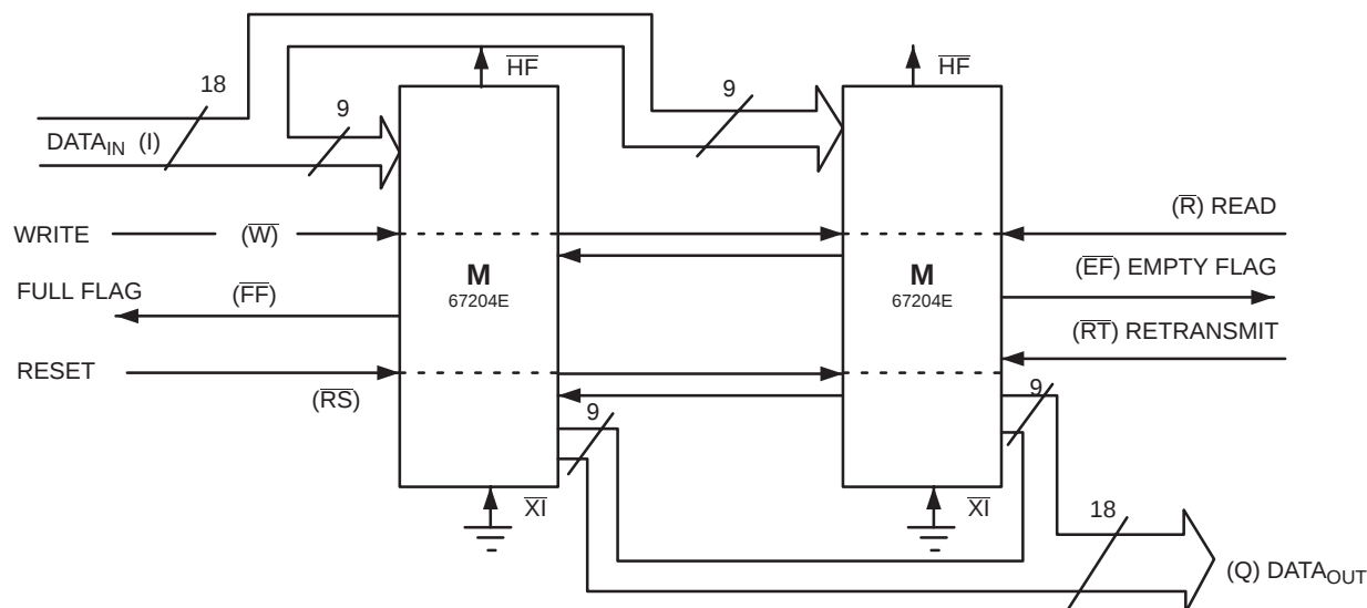
Figure 3. Block Diagram of 4096 \times 18 FIFO Memory Used in Width Expansion Mode.
