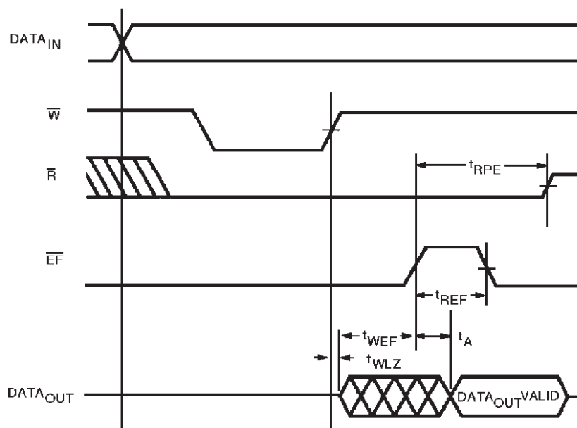
Figure 17. Read Data Flow – Through Mode.
