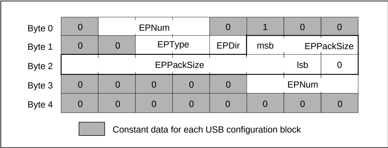
Figure 6-40 USB Configuration Block
