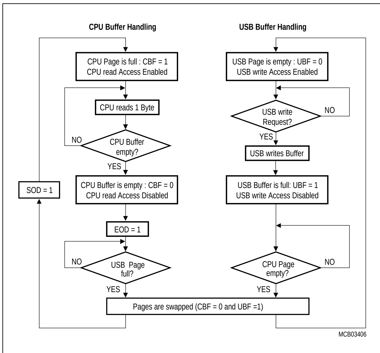
Figure 6-33 USB Write Access in Dual Buffer Mode - Buffer Handling
