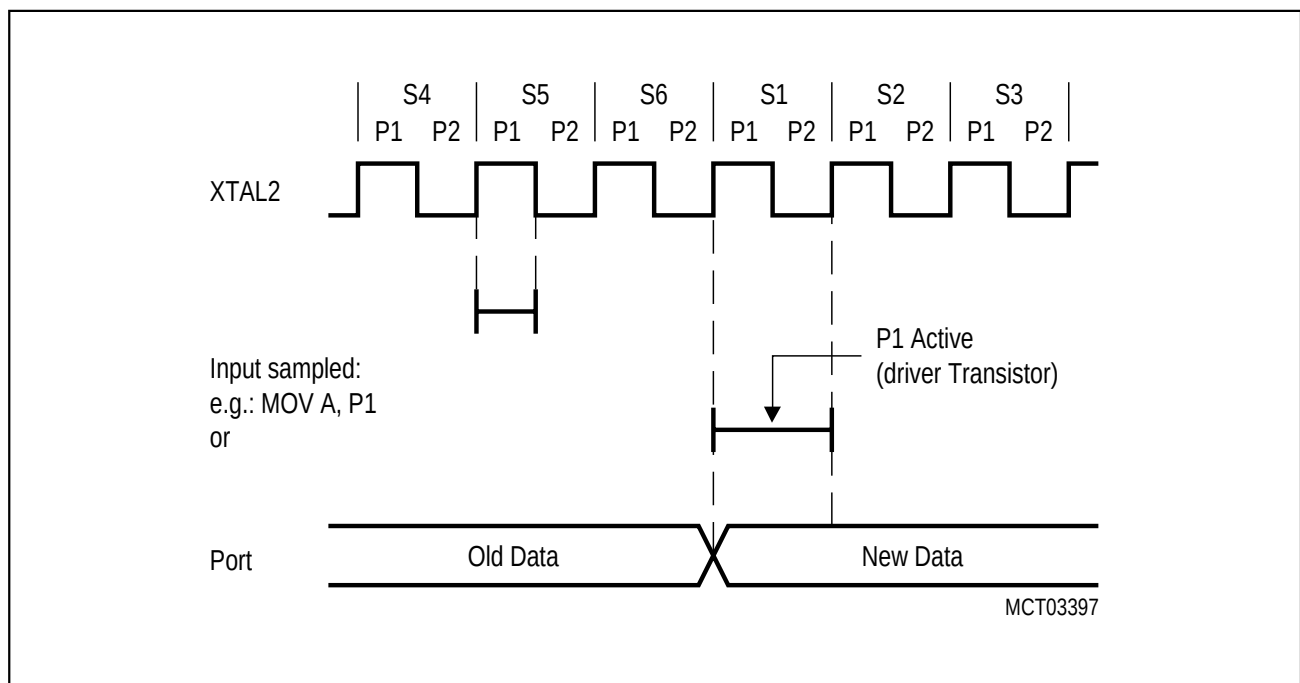
Figure 6-16 Port Timing
