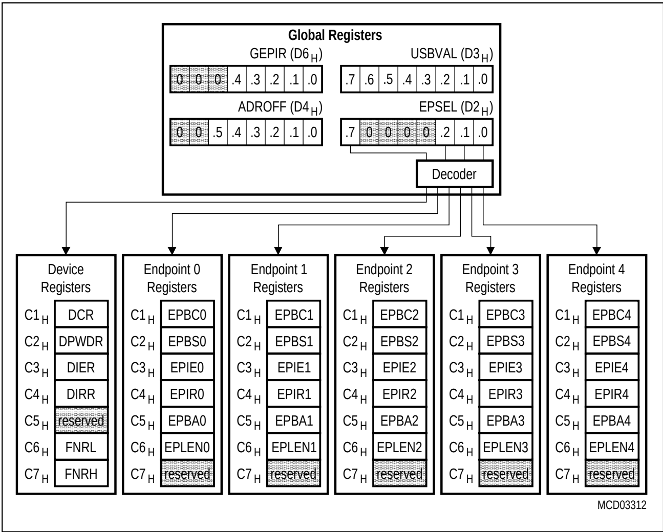
Figure 6-41 Register Structure of the USB Module
