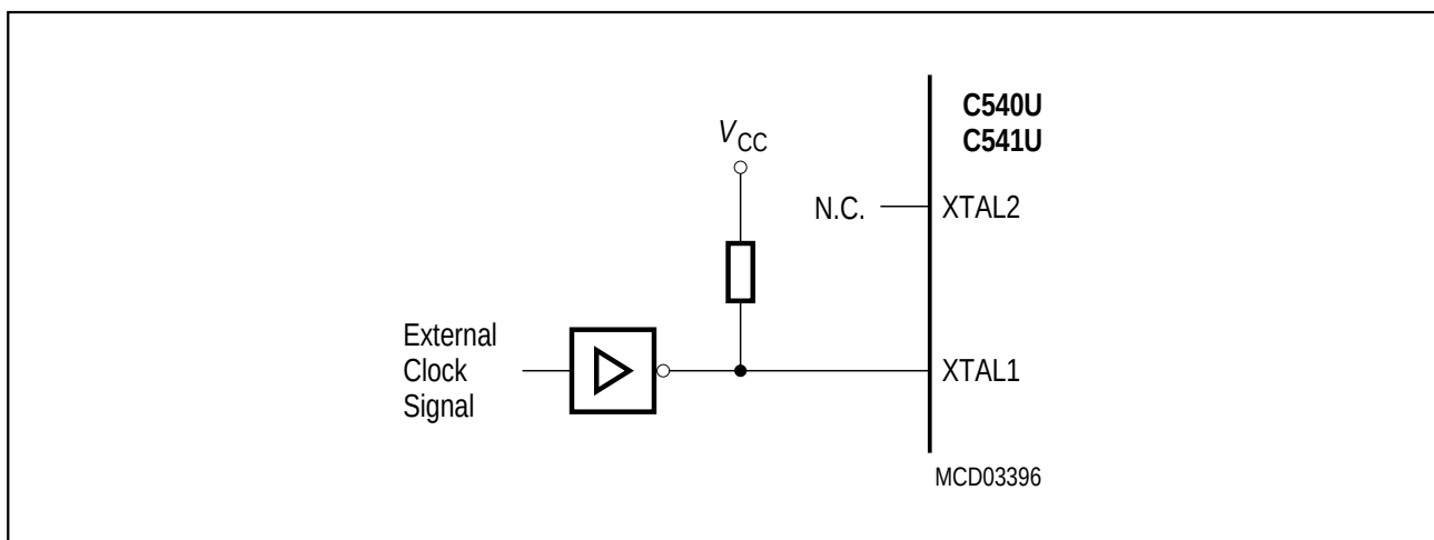
Figure 5-9 External Clock Source
