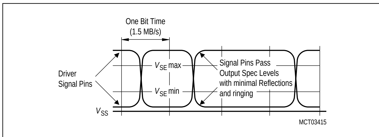
Figure 6-44 Low Speed USB Driver Signal Waveforms
