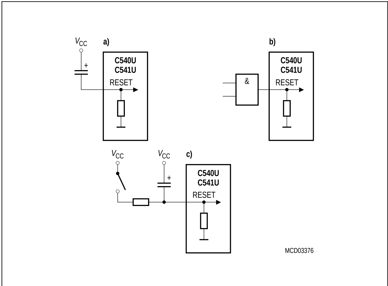
Figure 5-3 Reset Circuitries
