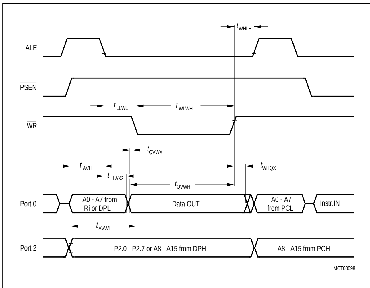
Figure 11-14 Data Memory Write Cycle
