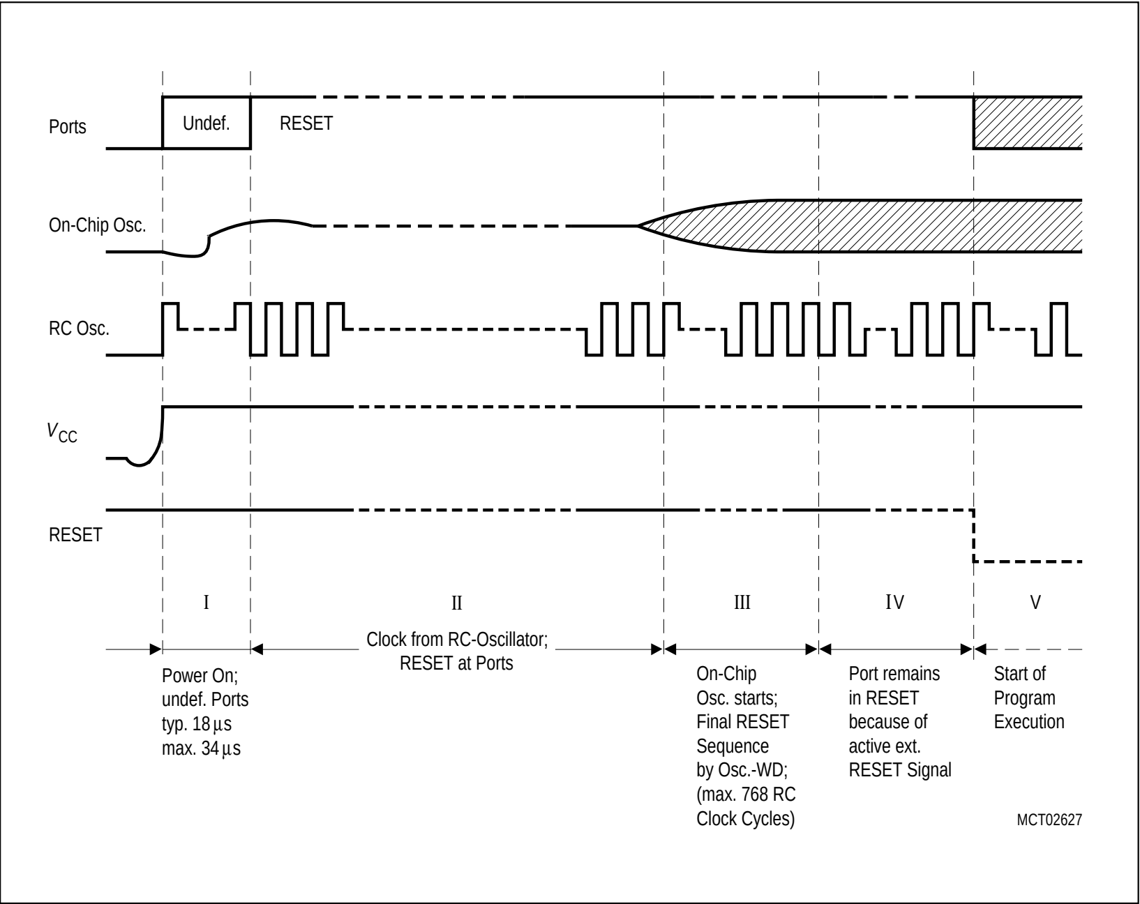
Figure 5-4 Power-On Reset of the C541U
