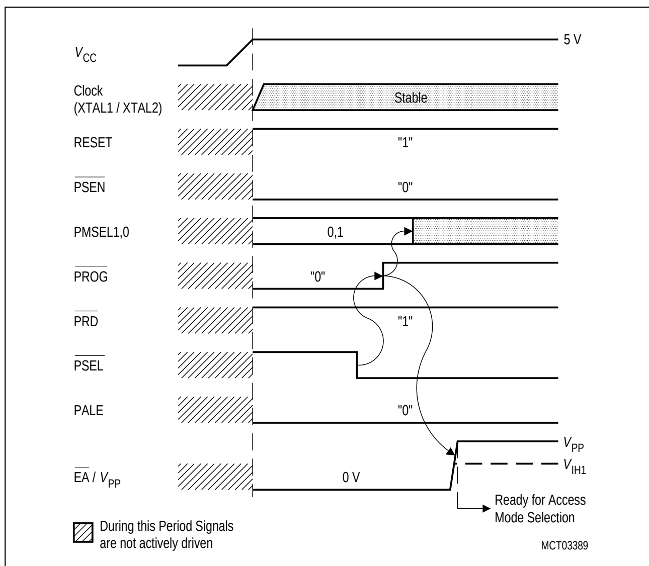
Figure 10-5 Basic Programming Mode Selection
