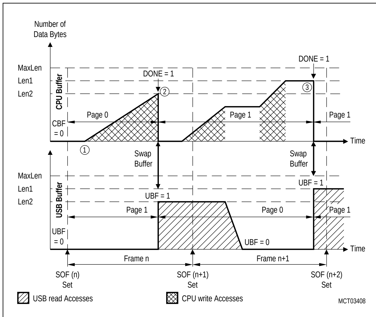
Figure 6-35 Dual Buffer Mode USB Read Access : Buffer Switching by Setting Bit DONE
