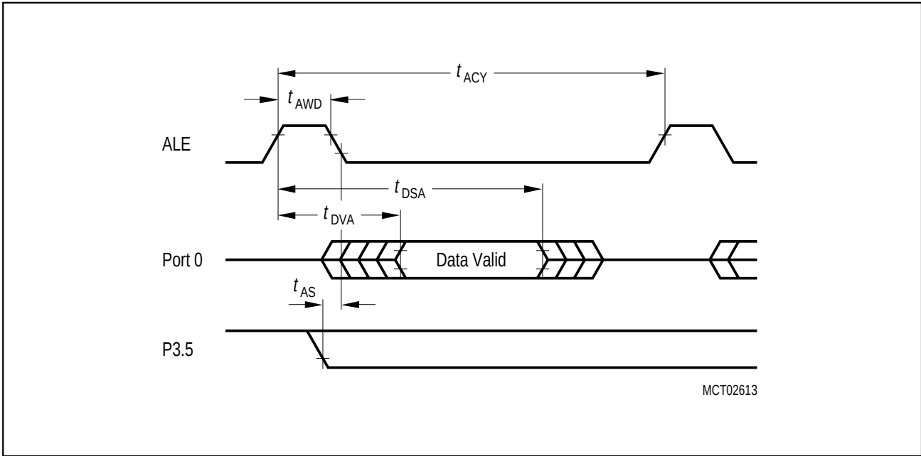
Figure 11-22 OTP Verification Mode for Protection Level 1
