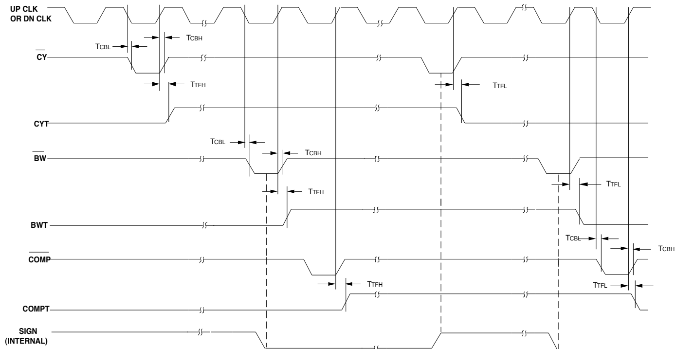
FIGURE 3. CLOCK TO \overline{\text{CY}} /BW OUTPUT PROPAGATION DELAYS
