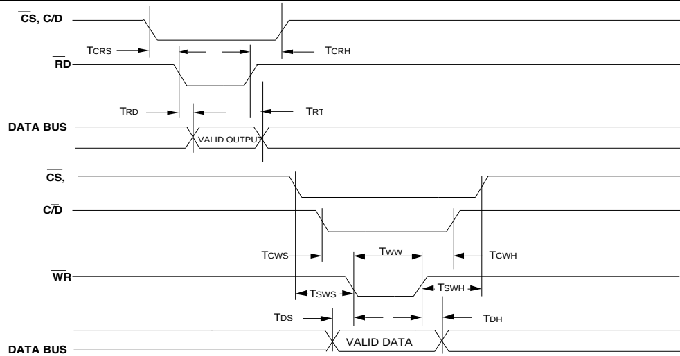
FIGURE 4. READ/WRITE CYCLES
