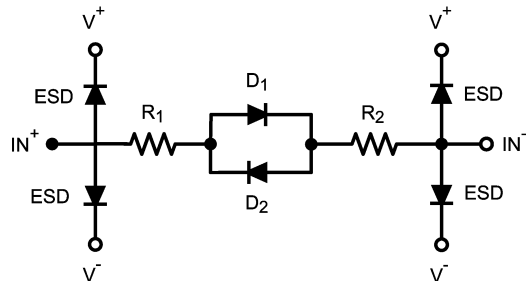
FIGURE 5. Input of LMP7701
