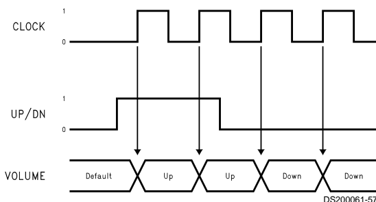
FIGURE 2. Timing Diagram
