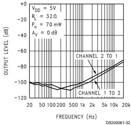
Channel Separation
