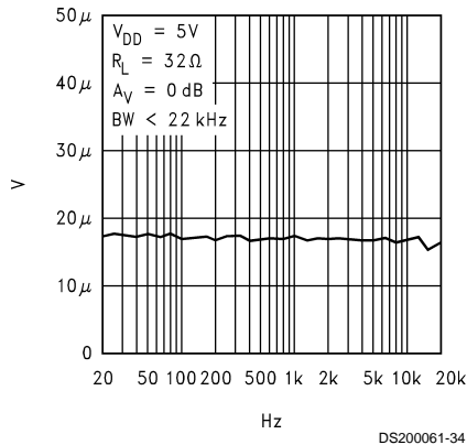
Noise Floor
