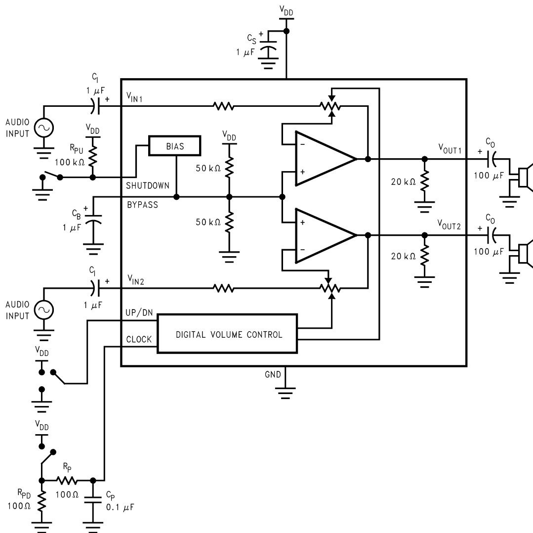
FIGURE 3. Demoboard Schematic
