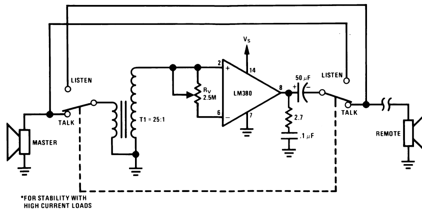
Intercom
