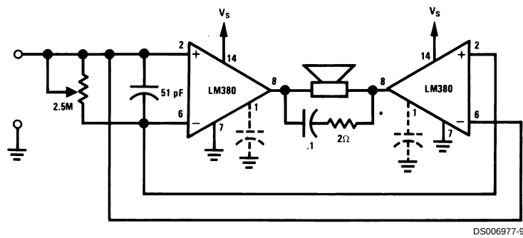
Bridge Amplifier
