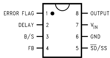
8-Lead DIP (N)
