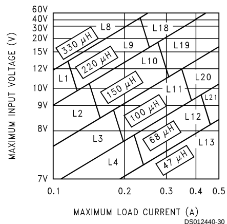
FIGURE 4. LM2597/LM2597HV-5.0
