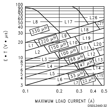
FIGURE 6. LM2597/LM2597HV-ADJ
