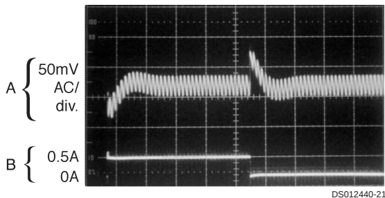
Load Transient Response for Continuous Mode
