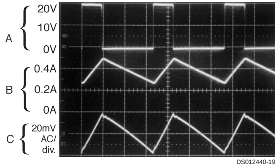
Continuous Mode Switching Waveforms
