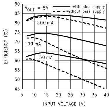
FIGURE 24. Effects of Bias Supply Feature on 5V Regulator Efficiency
