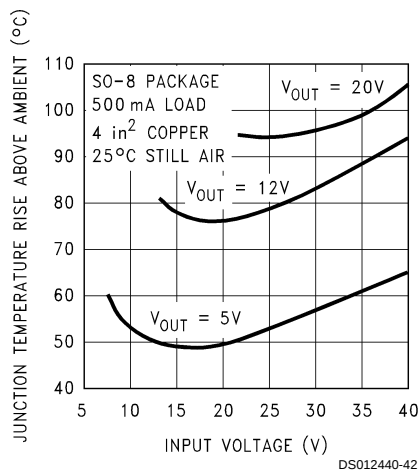
FIGURE 22. Junction Temperature Rise, DIP-8
