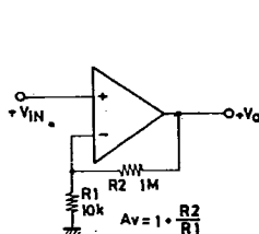
Non-inverting DC amplifier
