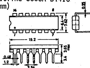
Case Outline 3003A-D14IC (unit:mm)
