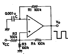
Square wave oscillator
