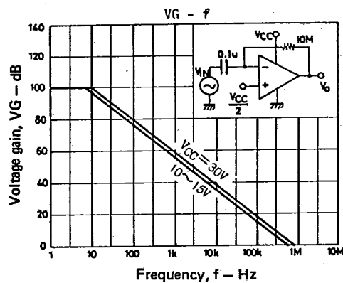
Inverting AC amplifier
