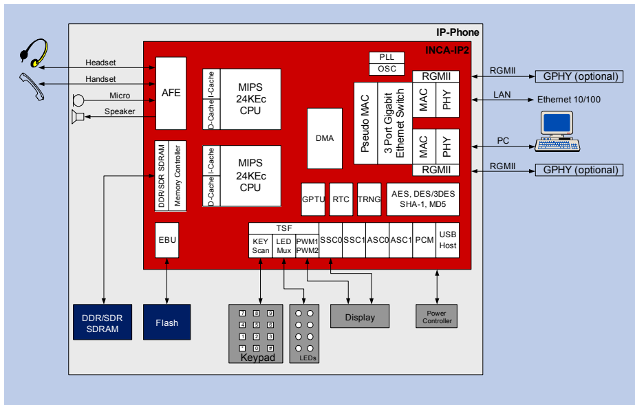
INCA-IP2 Block Diagram
