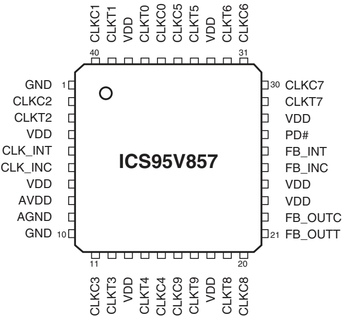
40-Pin MLF
