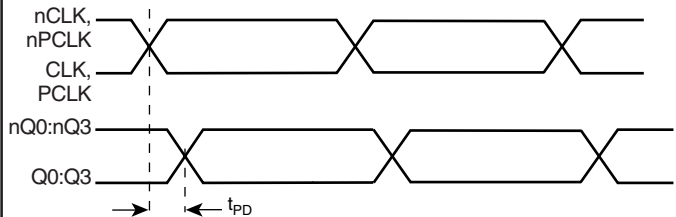
PROPAGATION DELAY
