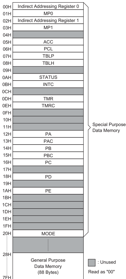
RAM Mapping
