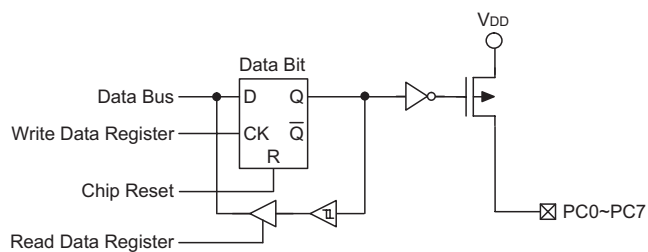
PC Output Ports
