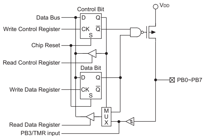
PB Input/Output Ports
