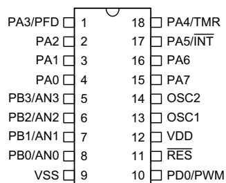
HT46R47 - 18 DIP/SOP
