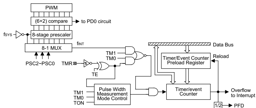
Timer/event counter
