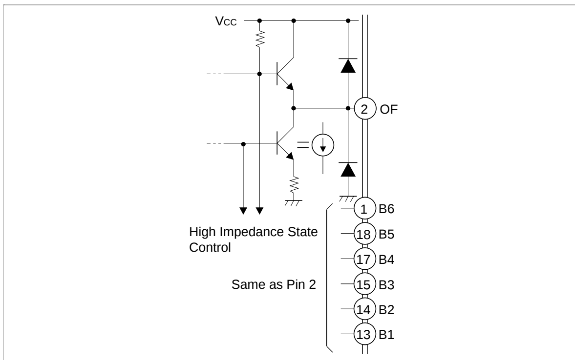
Figure 4 Digital Output
