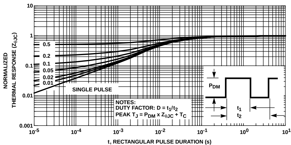
FIGURE 7. NORMALIZED MAXIMUM TRANSIENT THERMAL RESPONSE
