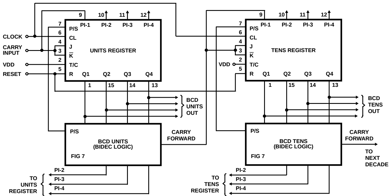
FIGURE 12. BINARY-TO-BCD CONVERTER
