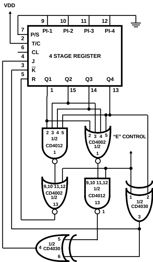
FIGURE 11(a). DOUBLE SEQUENCE GENERATOR
