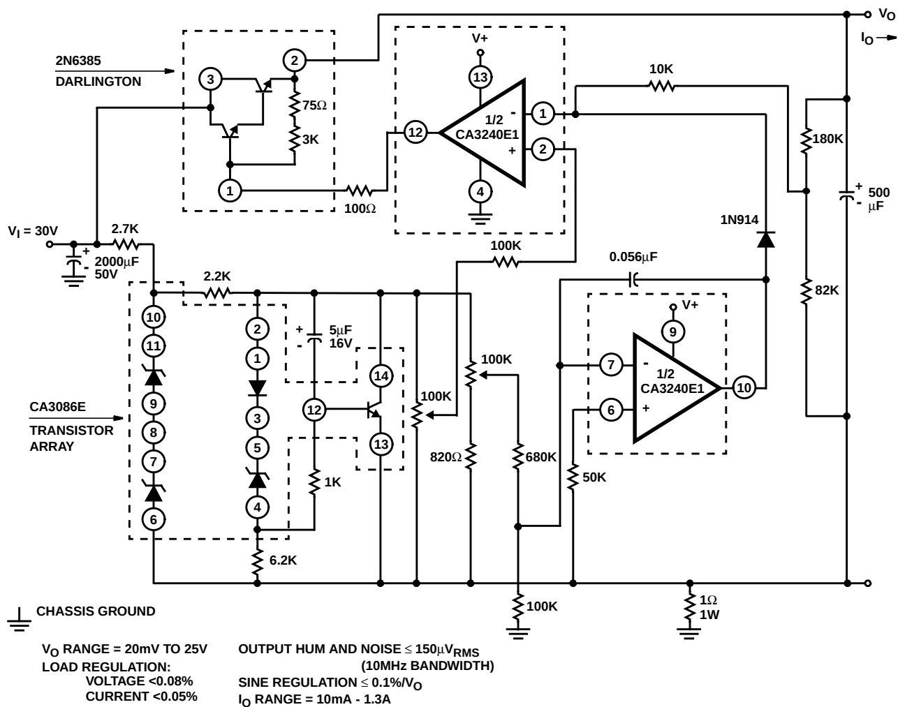
FIGURE 8. CONSTANT-VOLTAGE/CONSTANT-CURRENT POWER SUPPLY
