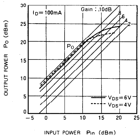
P_o vs. P_{in} ( f = 8\text{ GHz} )
