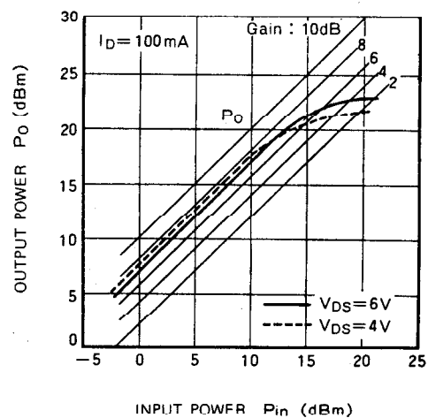
P_o vs. P_{in} ( f = 12\text{ GHz} )
