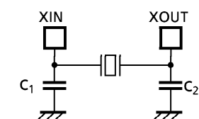
(1) High-frequency Oscillation
