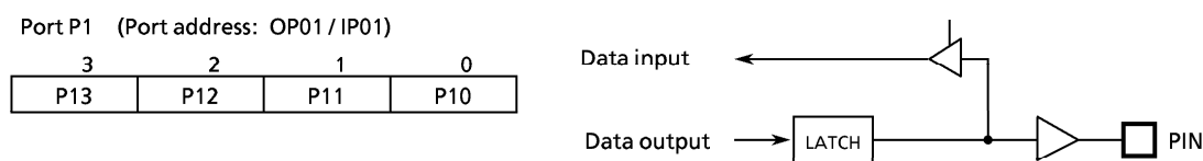
Figure 2-2. Ports P1
