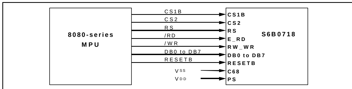
Figure 46. In Case of Interfacing with 8080-series (PS = "H", C68 = "L")
