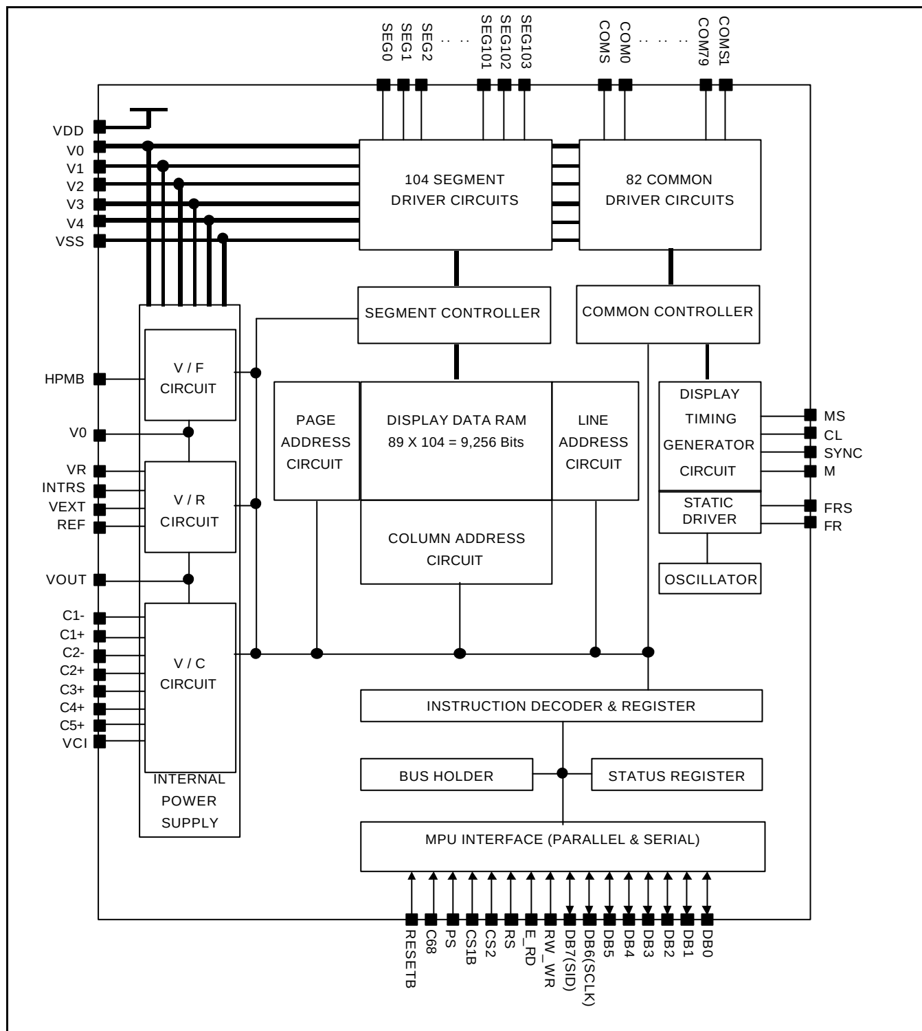
Figure 1. Block Diagram
