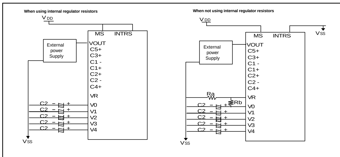
Figure 25. When Using some LCD Power Circuits (V/C: OFF, V/R: ON, V/F: ON)
