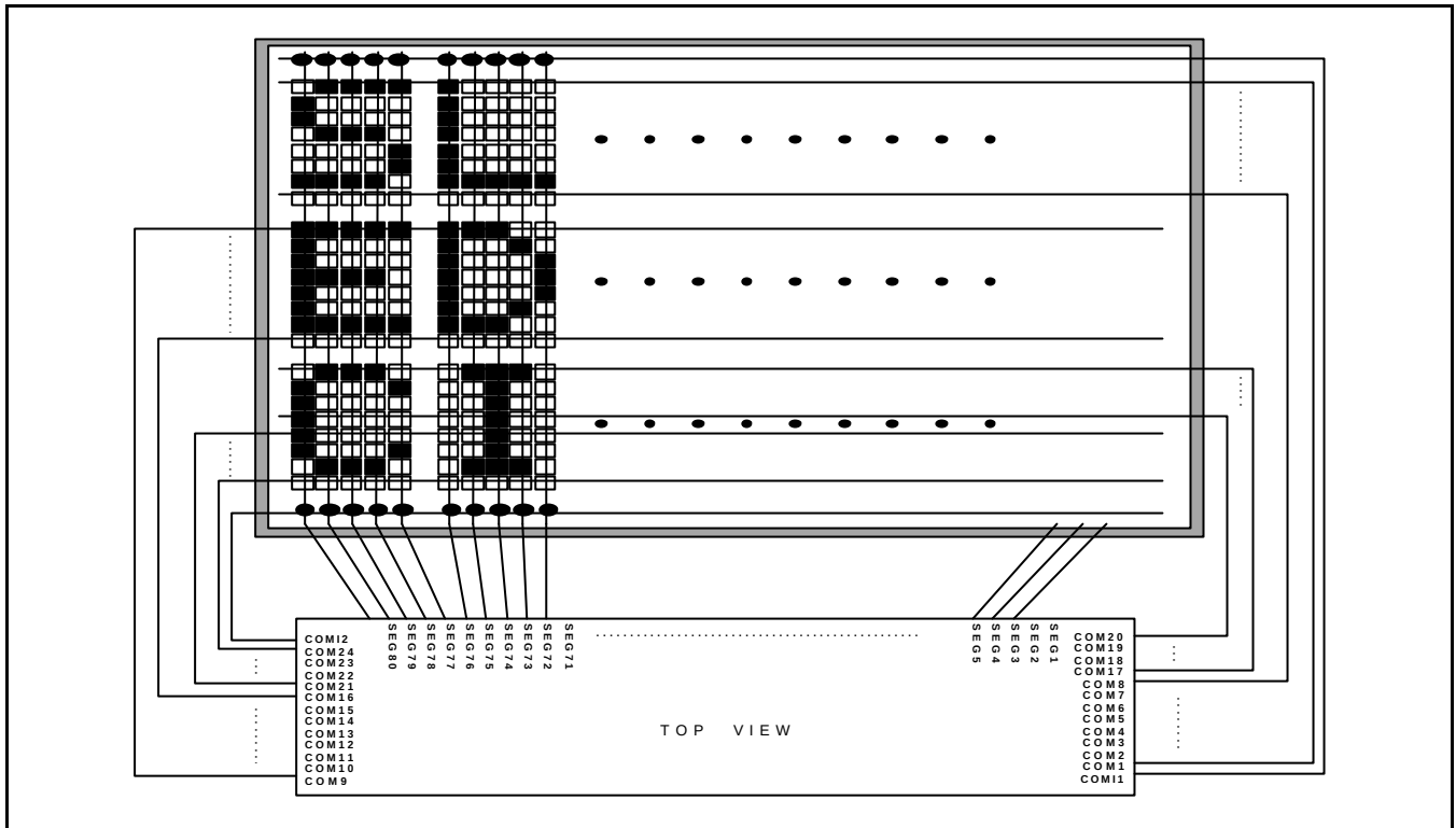
Chip Top &amp; Upper View (S bit = "1", DIRS = "0")
