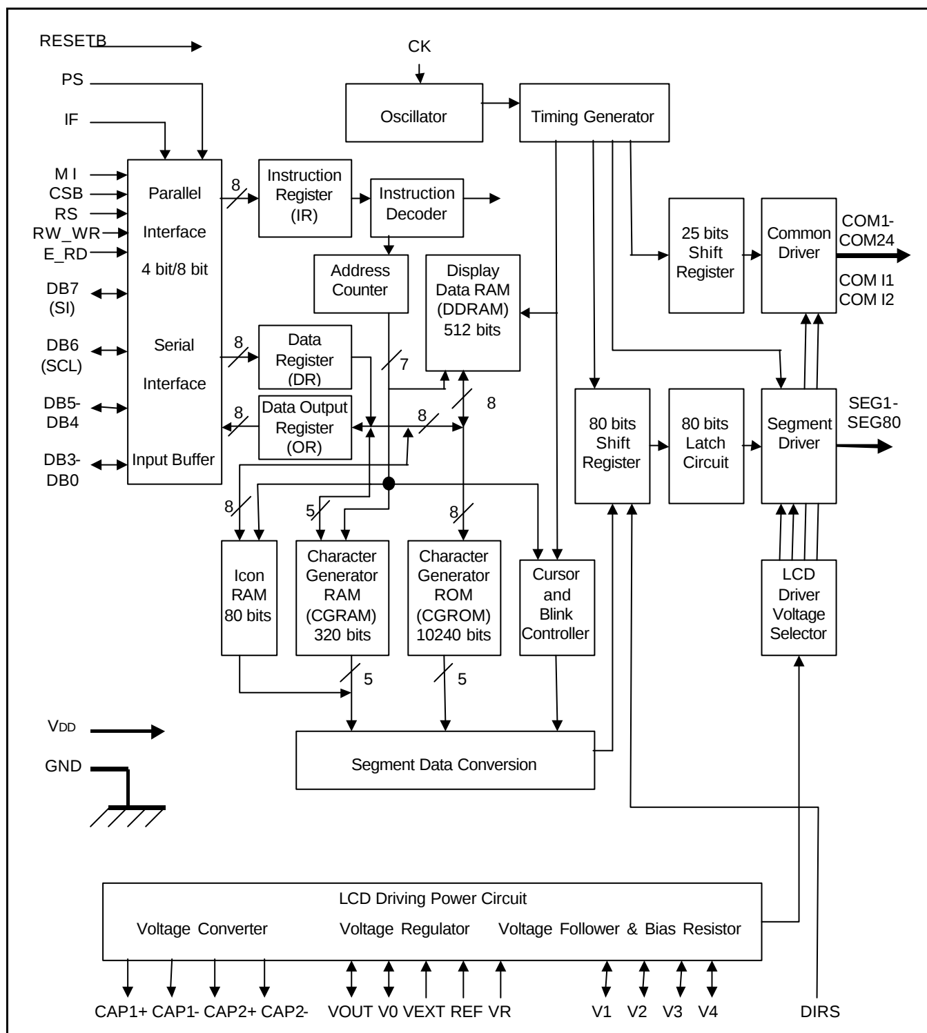
Figure 1. Block Diagram
