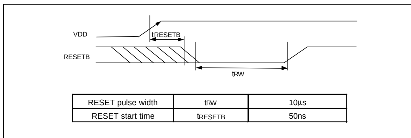
Figure 17. RESET Timing
