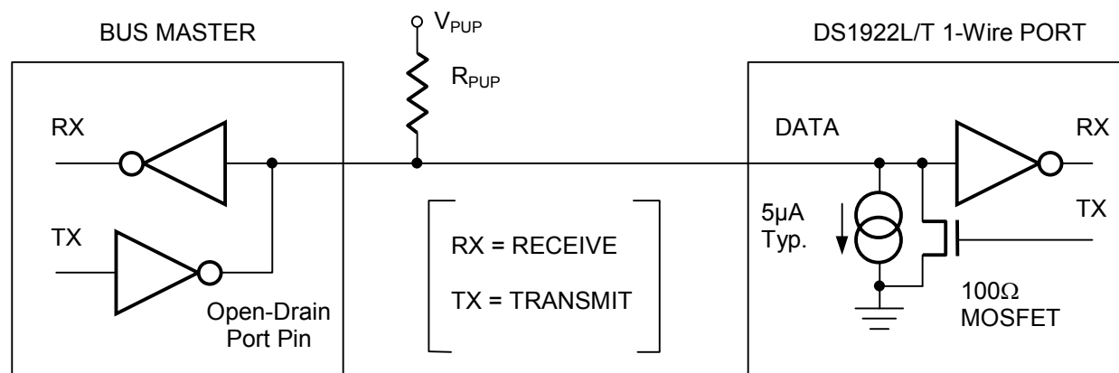
Figure 10. Hardware Configuration
