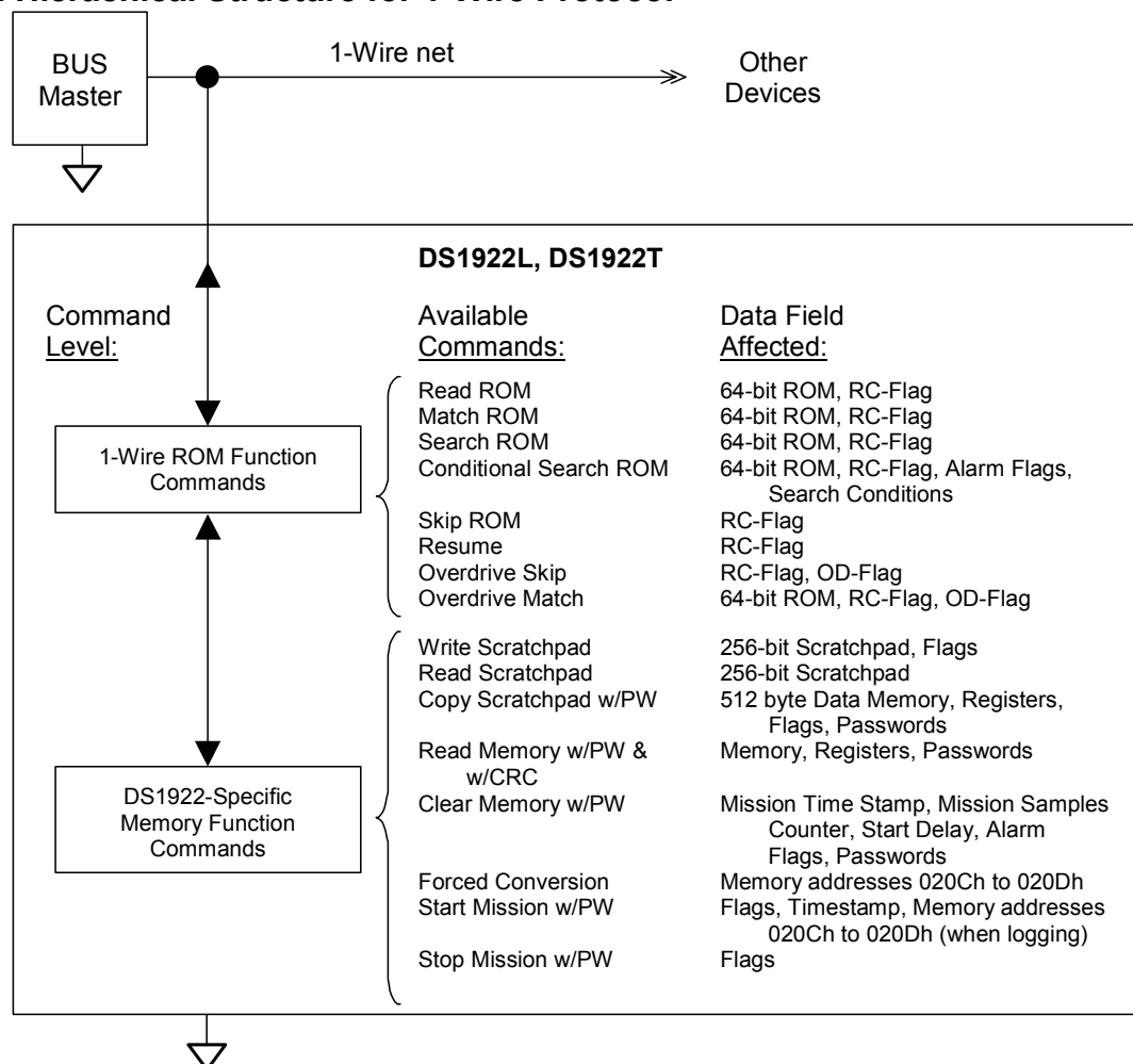
Figure 2. Hierarchical Structure for 1-Wire Protocol
