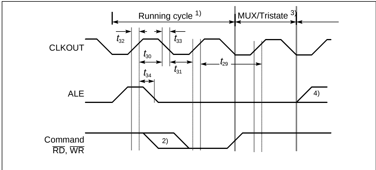
Figure 15 CLKOUT Timing
