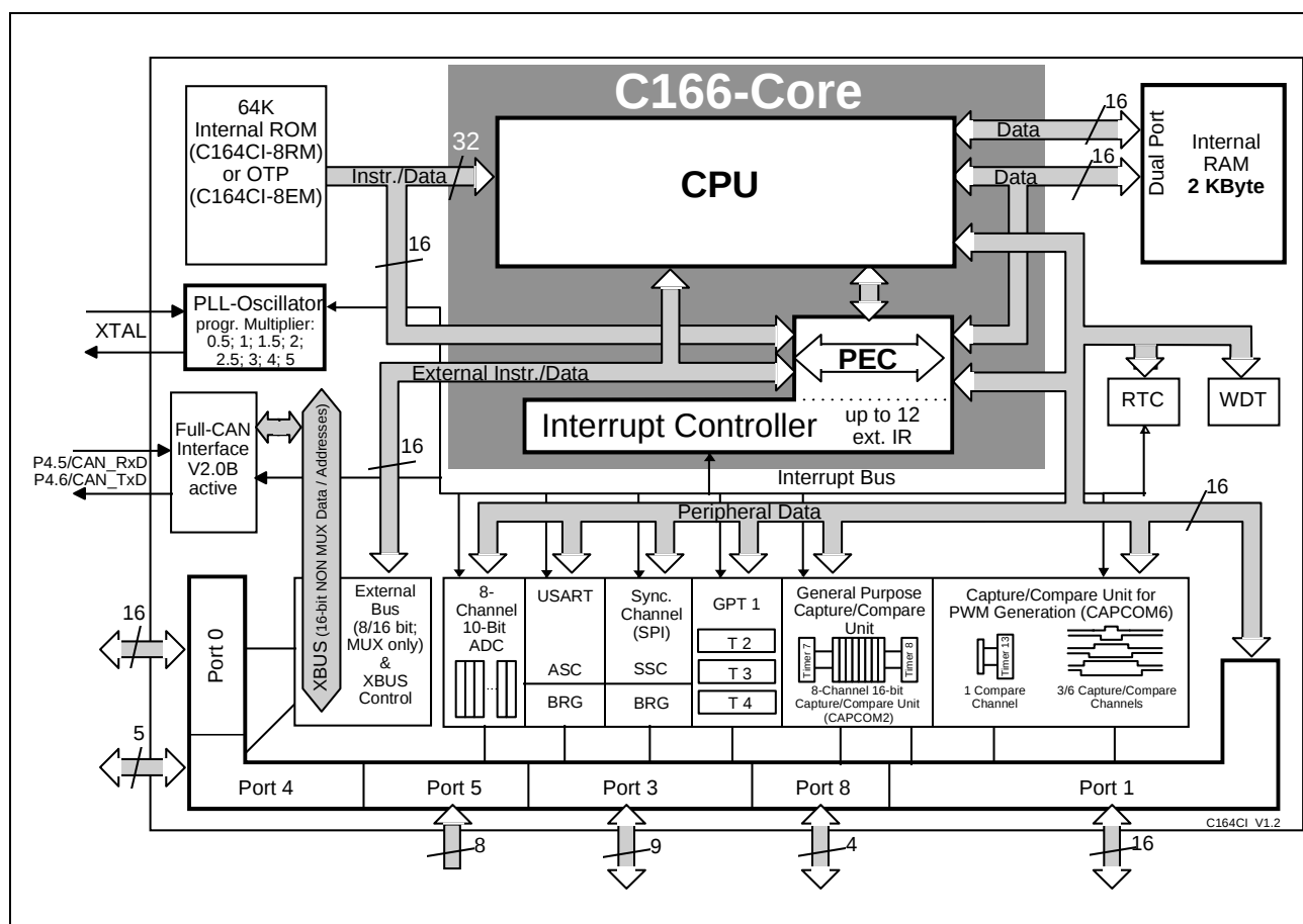
Figure 3 Block Diagram
