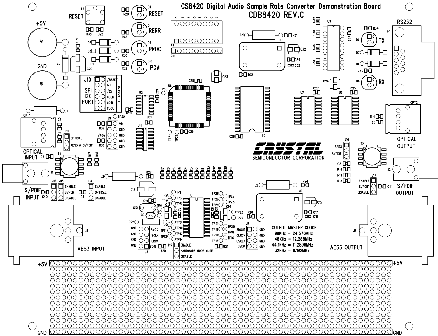
Figure 6. Silkscreen
