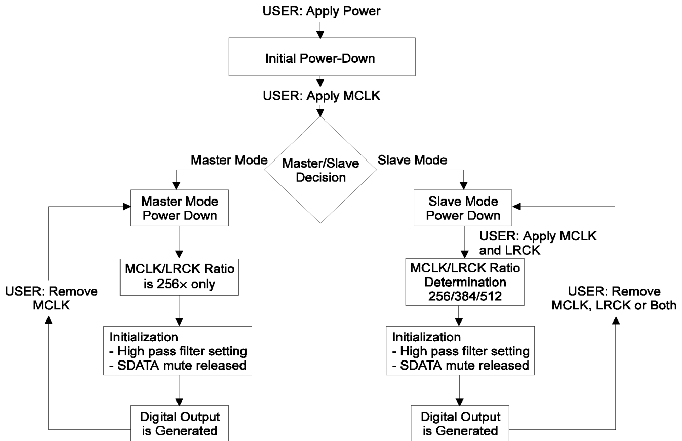
Figure 4. CS5330A/31A Initialization and Power-Down Sequence
