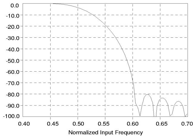
Figure 8. CS5330A/31A Digital Filter Transition Band
