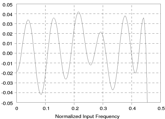
Figure 7. CS5330A/31A Digital Filter Passband Ripple
