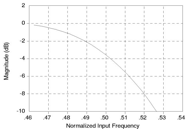
Figure 6. CS5330A/31A Digital Filter Transition Band
