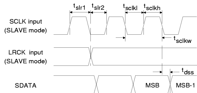
SCLK to LRCK & SDATA - SLAVE mode (CS5331A)
