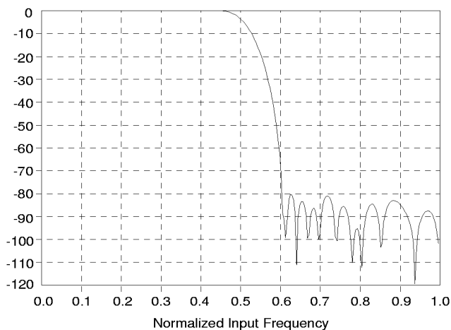
Figure 5. CS5330A/31A Digital Filter Stopband Rejection
