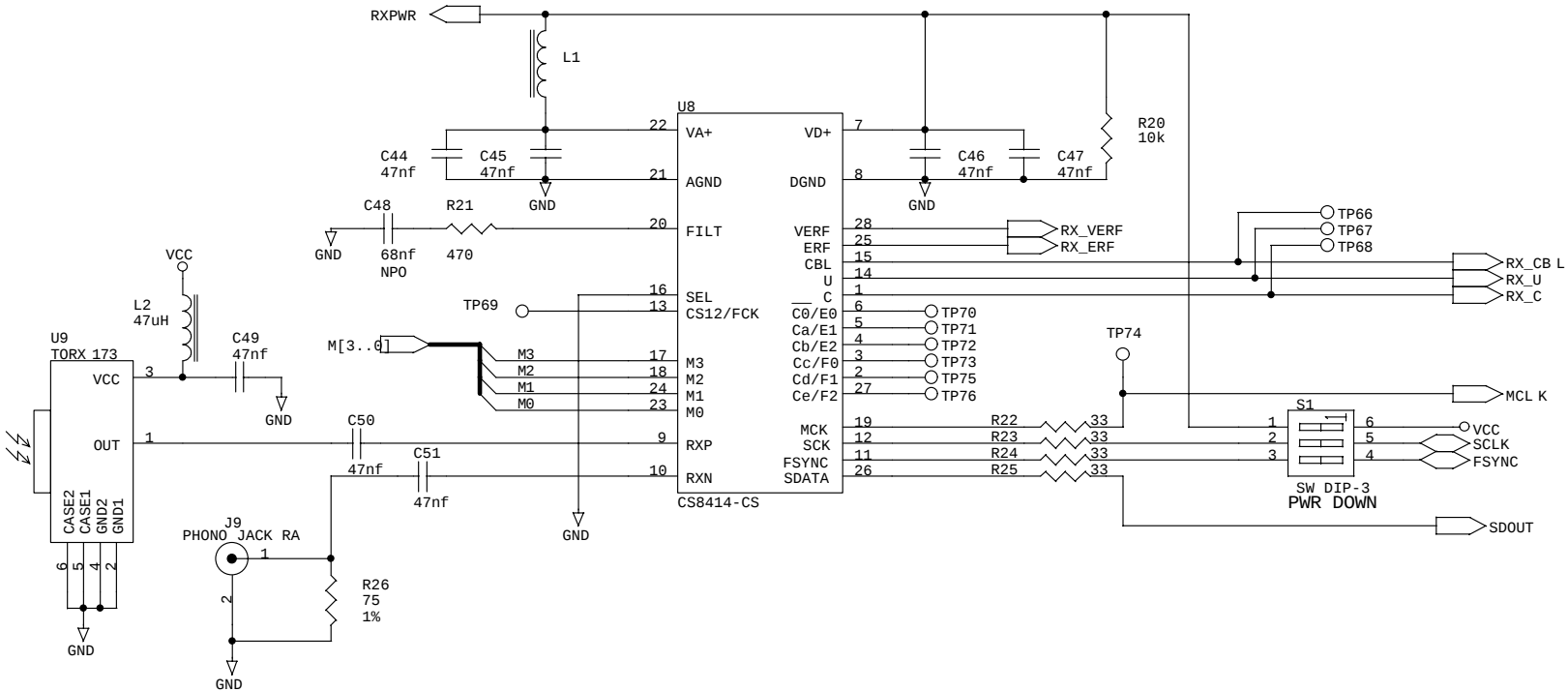
Figure 16. CS8414 Digital Audio Receiver
