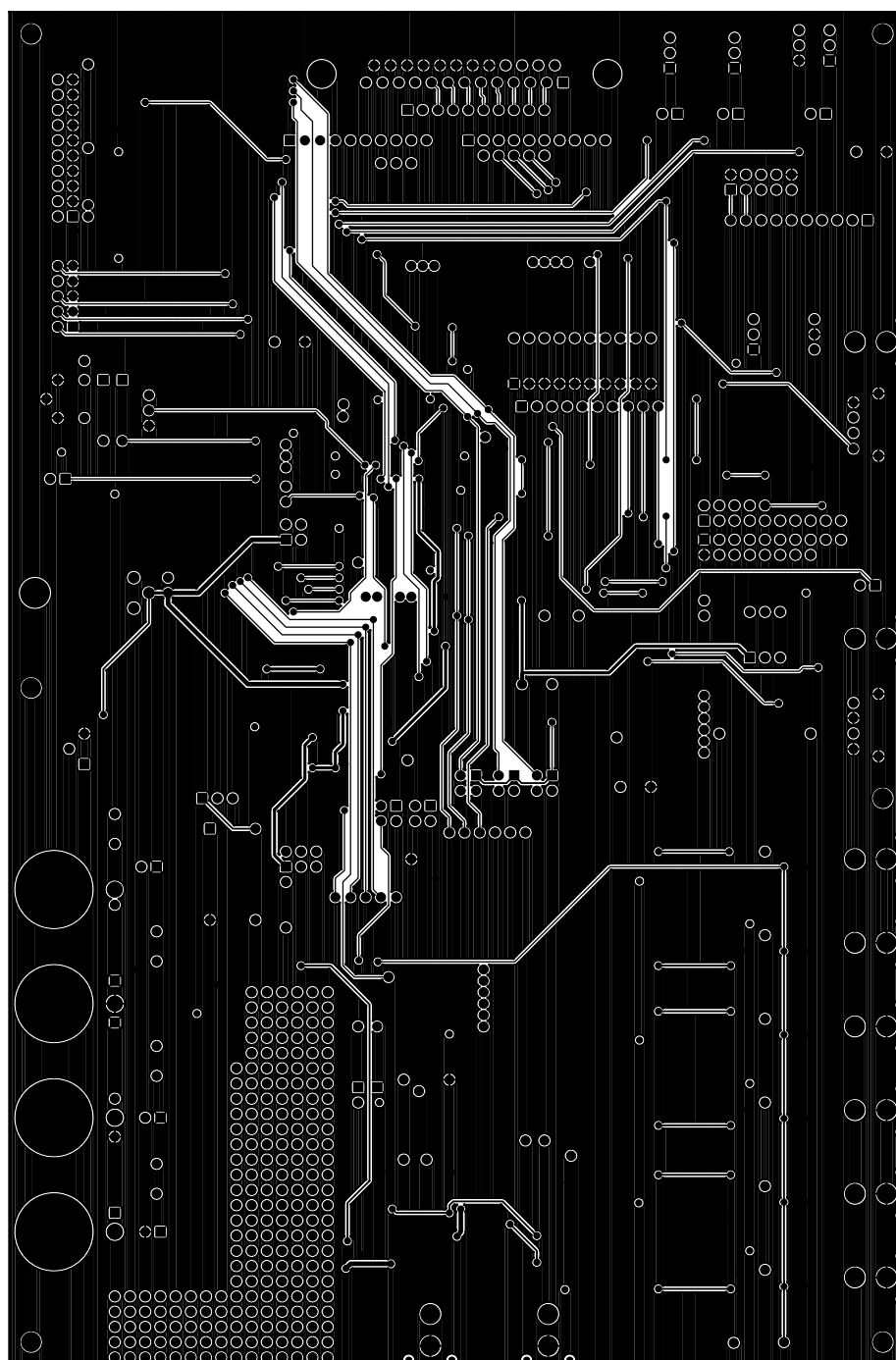
Figure 22. Bottom Side
