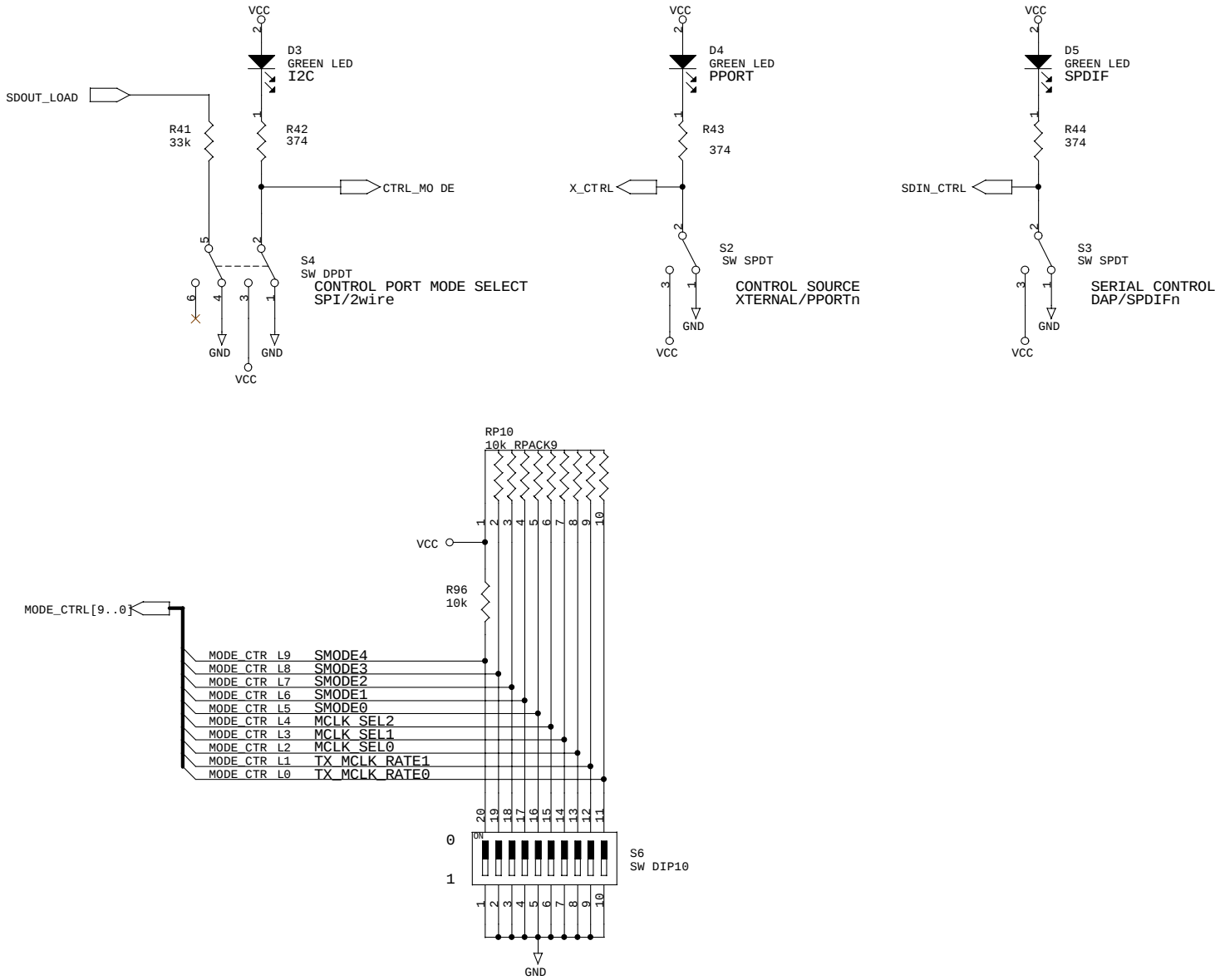
Figure 3. External Control
