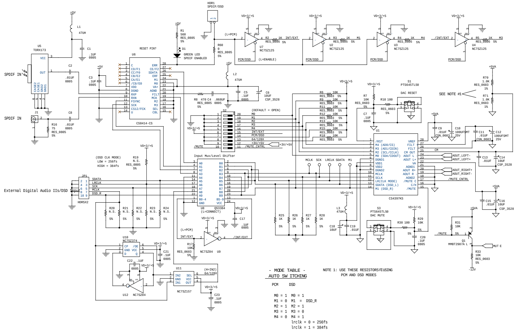
Figure 1. System Schematic
