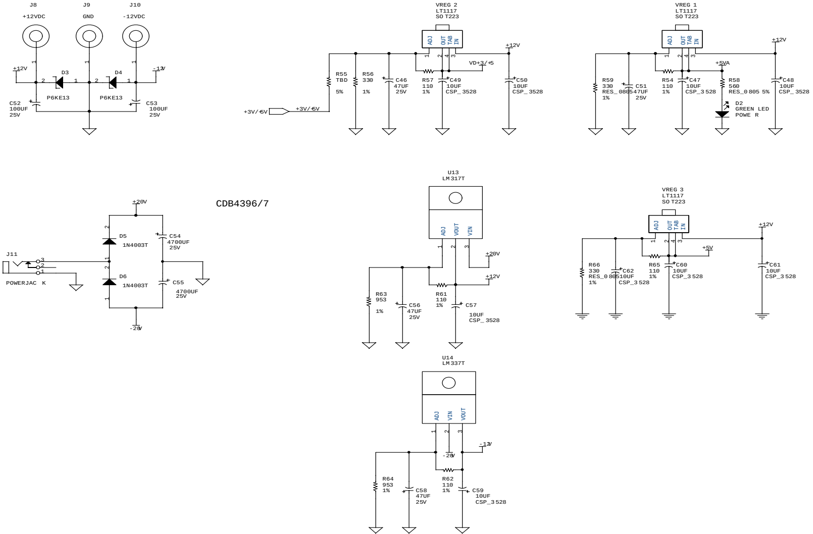
Figure 3. Power Supply
