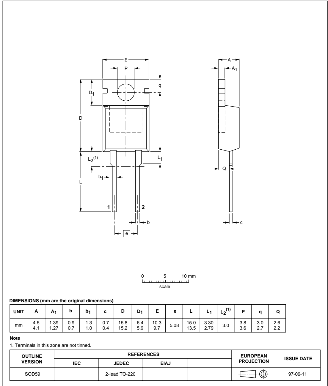
Fig. 12. TO220AC; pin 1 connected to mounting base.
