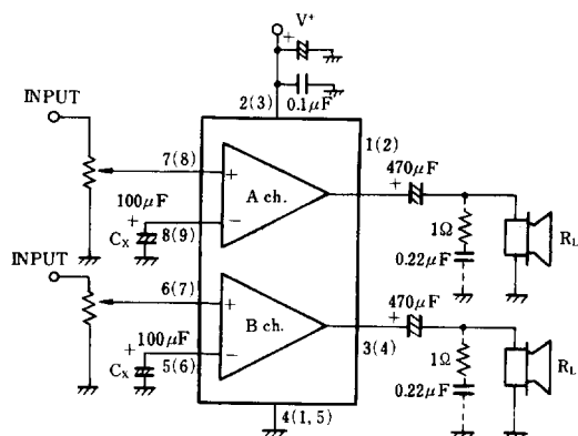
Fig.2 Stereo Configuration
