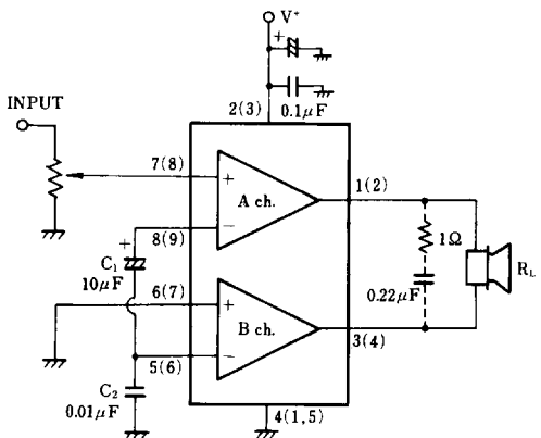
Fig.1 BTL Configuration
