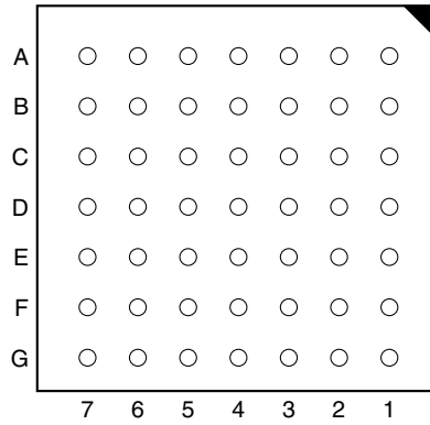
ATF1504AE(L) 49-ball 0.8 mm Pitch Bottom View
