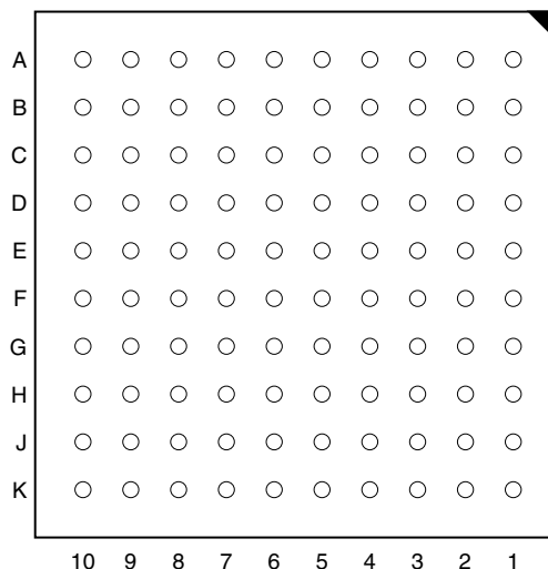
ATF1504AE(L) ATF1508AE(L) ATF1516AE(L) 100-ball 1.0 mm Pitch – Bottom View
