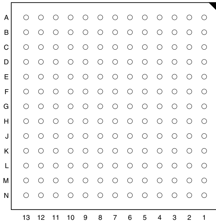
ATF1508AE(L) 169-ball 0.8 mm Pitch Bottom View
