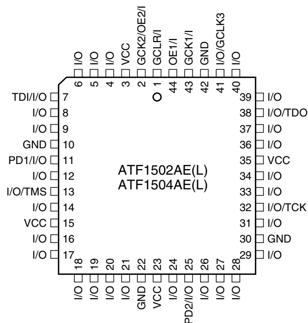
44-lead TQFP
