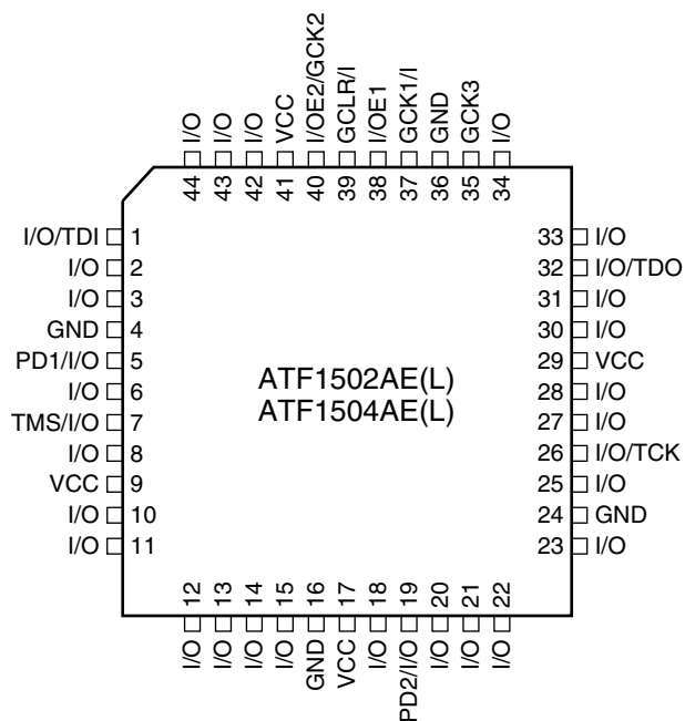
44-lead TQFP
