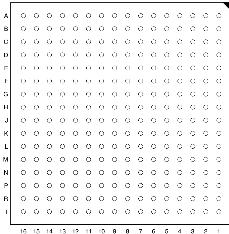
ATF1532AE(L) 256-ball 1.0 mm Pitch Bottom View
