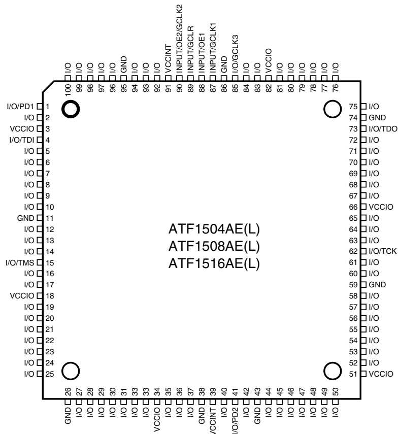
100-lead TQFP
