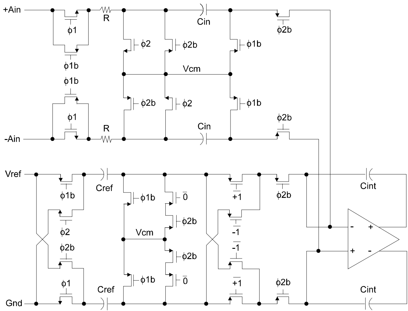
Figure 6. Switched-Capacitor Integrator Circuit
