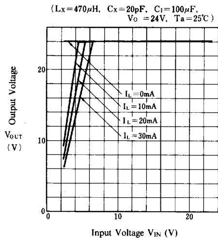
Output Voltage
