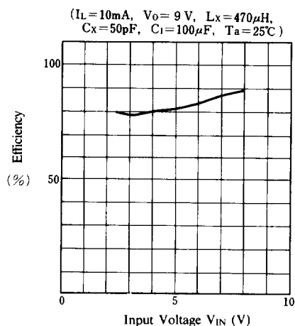
Efficiency
