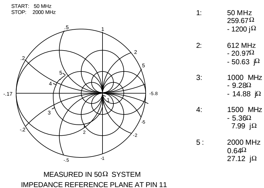
Figure 5: LO Impedance
