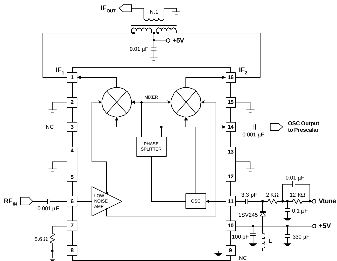
Figure 2: Test Circuit Schematic
