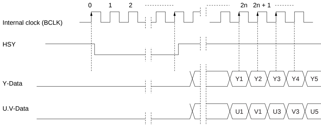
Fig. 25 YUV input timing when TEST[2] = L
