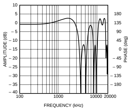
Gain-Phase Graphic
