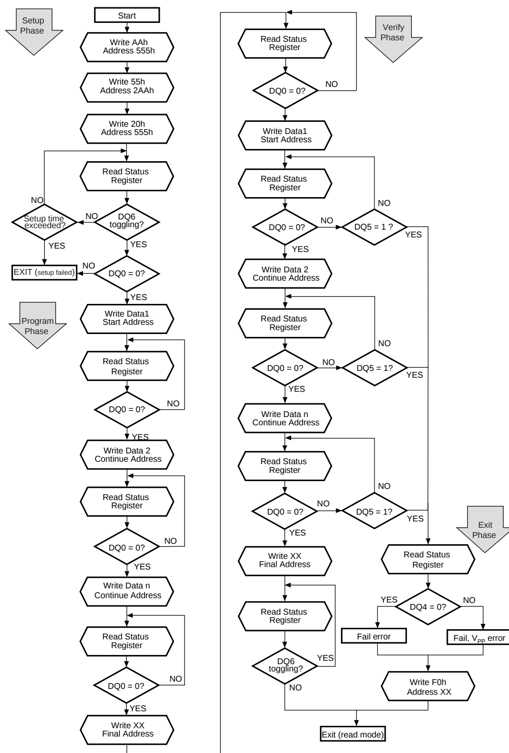
Figure 5. Multiple Word Program Flowchart
