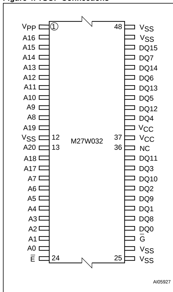
Figure 4. TSOP Connections
