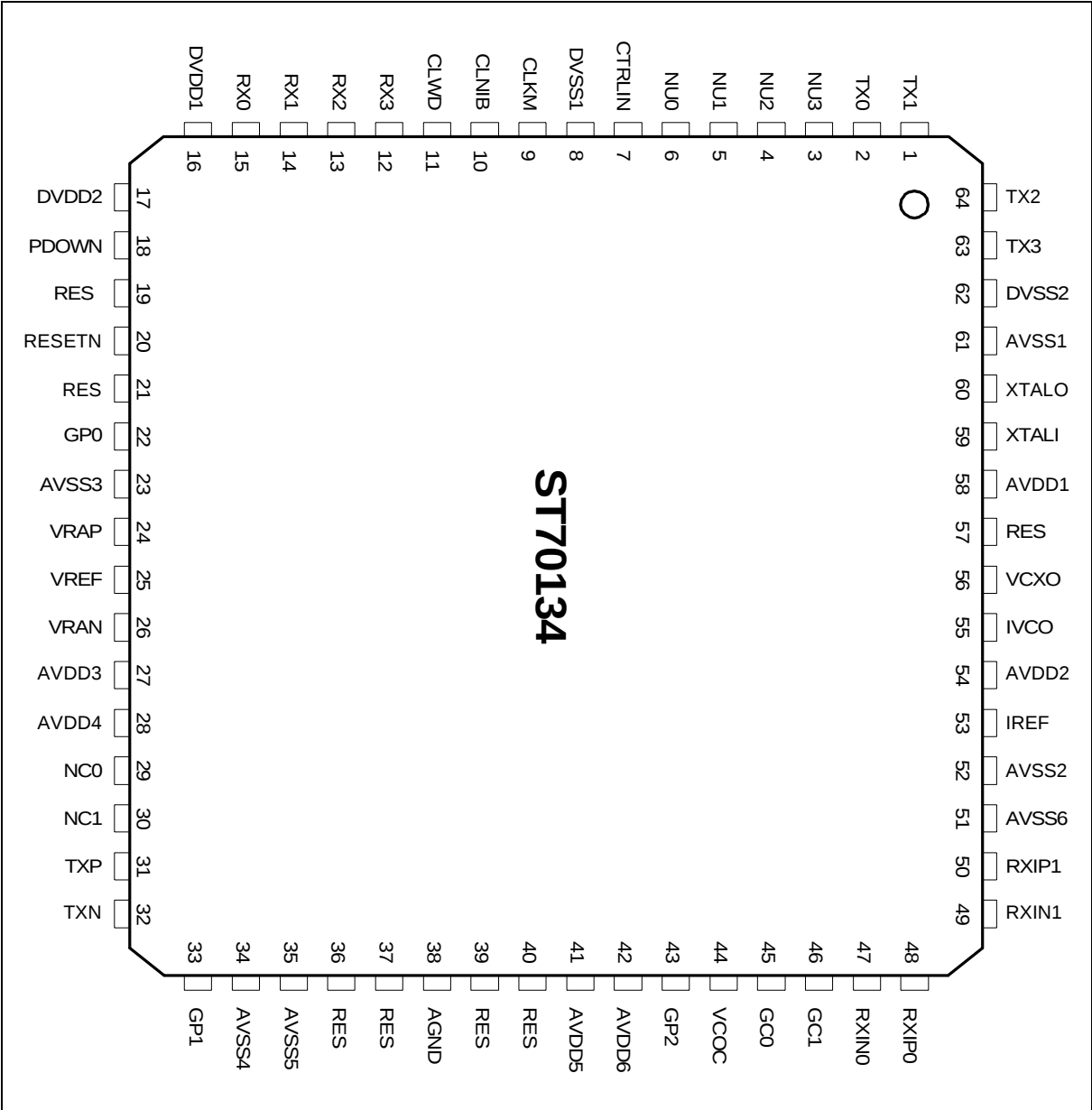
Figure 2 : Pin Connection
