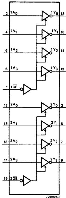
Fig.4 Functional diagram.
