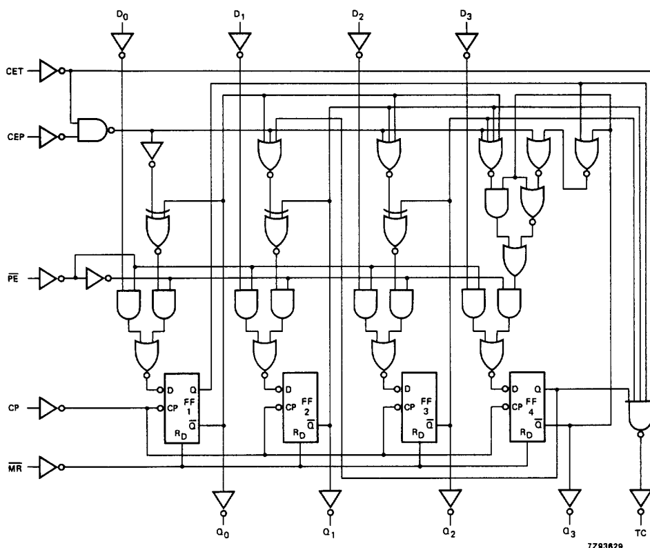
Fig.7 Logic diagram.
