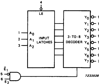
Fig.2 Logic symbol.
